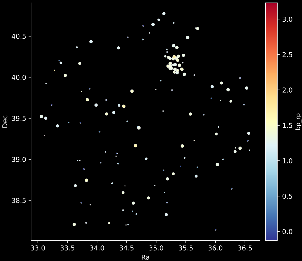
APOGEE DR17 Field: [N6819-RV_btx] Stars: 137
