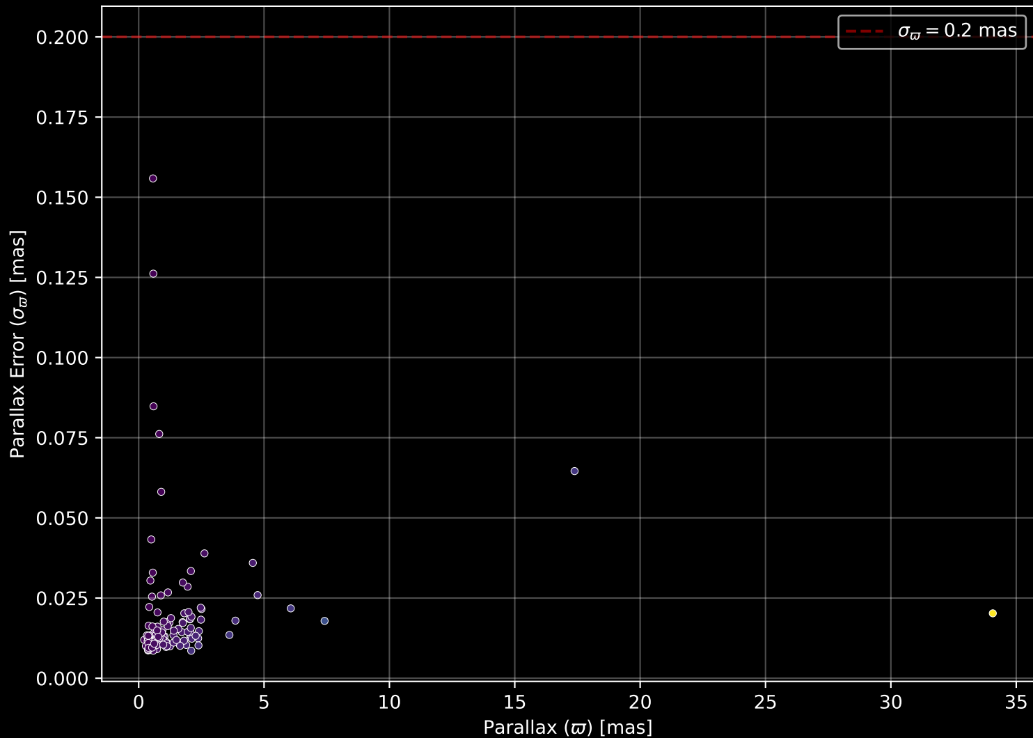
APOGEE DR17 Field: [N6819-RV_btx] Parallax Quality (n= 137)
