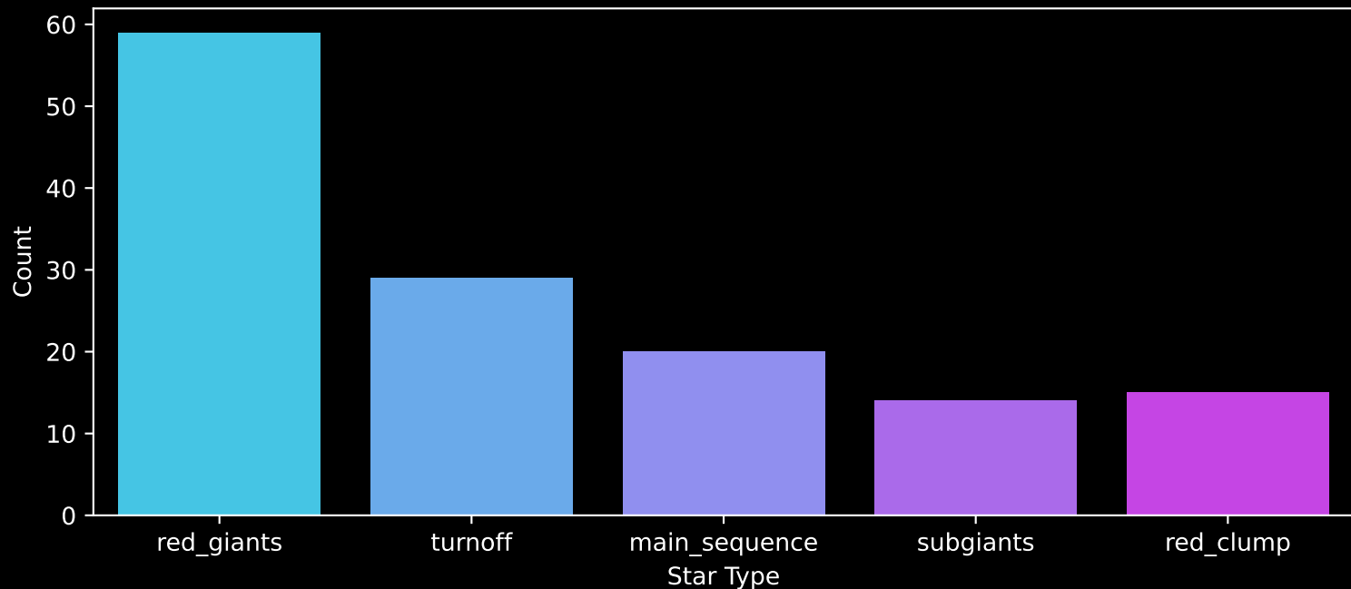
APOGEE DR17 Field: [N6819-RV_btx] Count plot of Star Type
