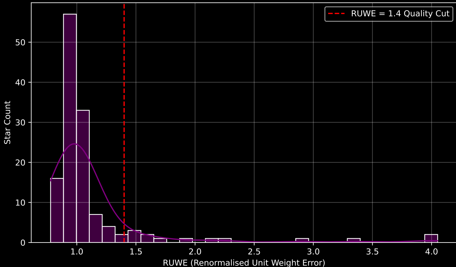
GAPOGEE DR17 Field [N6819-RV_btx] RUWE Distribution (n= 132)
