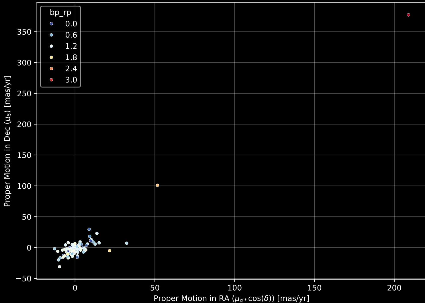
APOGEE DR17 Field: [N6819-RV_btx] Proper Motion Diagram (n= 137)
