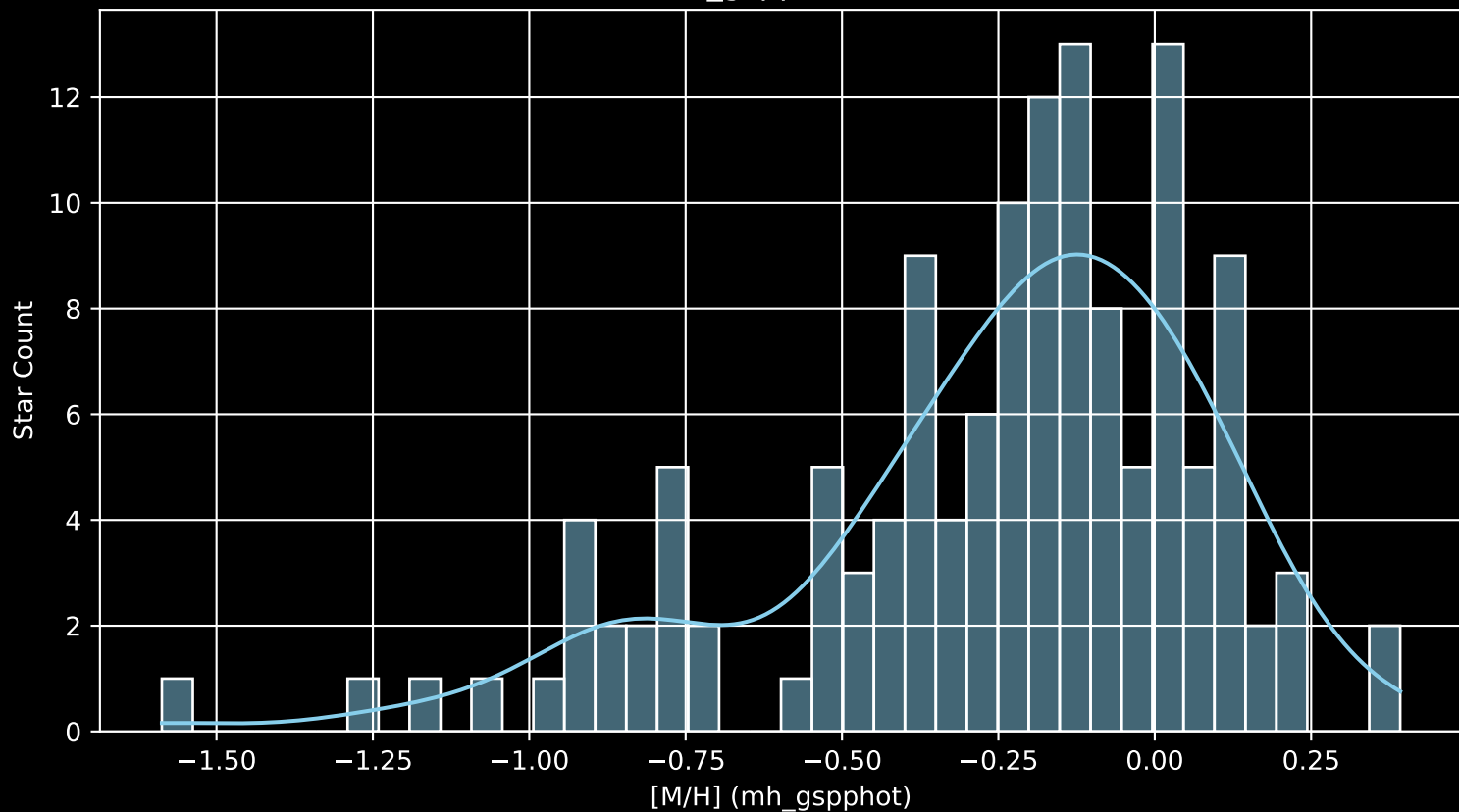
APOGEE DR17 Field: [N6819-RV_btx [M/H] (mh_gspphot) (n= 134)
